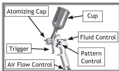
Figure 4. Controls.
