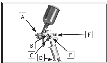
Figure 11. Lubrication points.
